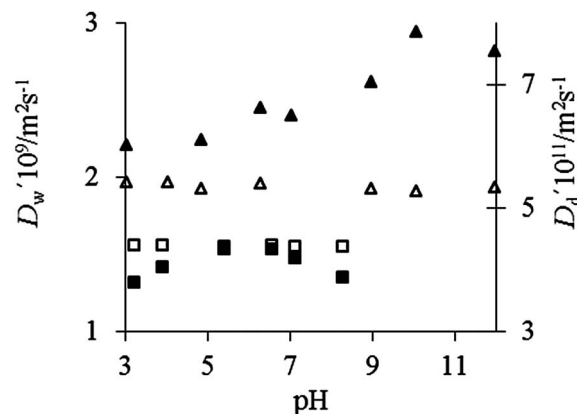
Fig. 5 The pH dependence of the diffusion coefficient of D 2 O ( D_w , left axis) and the dendrimers ( D_d , right axis). \square and \blacksquare show the diffusion of water and E5.SAH in the same solution respectively ( c = 0.41 \text{ mmol kg}^{-1} , T = 293 \text{ K} ) while \Delta and \blacktriangle show the diffusion water and E5.NH 2 in the same solution ( c = 0.37 \text{ mmol kg}^{-1} , T = 300 \text{ K} ) respectively.
